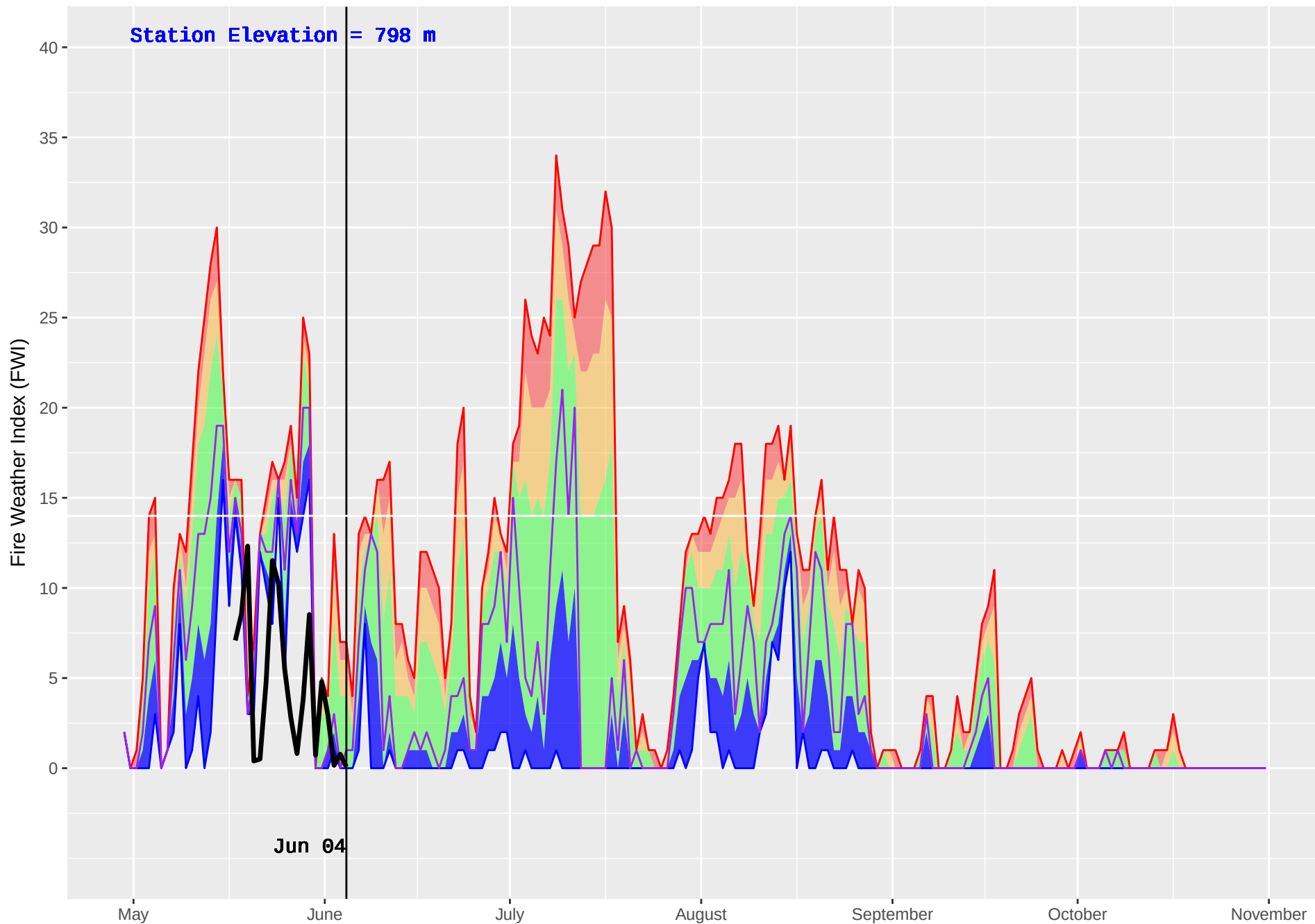
SEVEREID (1165) : Historical (2014–2016) and Current (2018) Noon Fire Weather Index (FWI)
