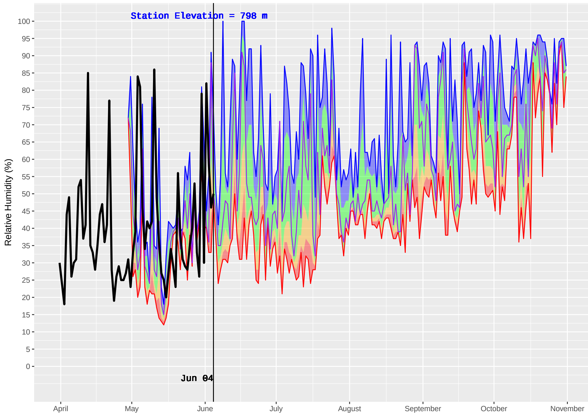
SEVEREID (1165) : Historical (2014–2016) and Current (2018) Noon Relative Humidity
