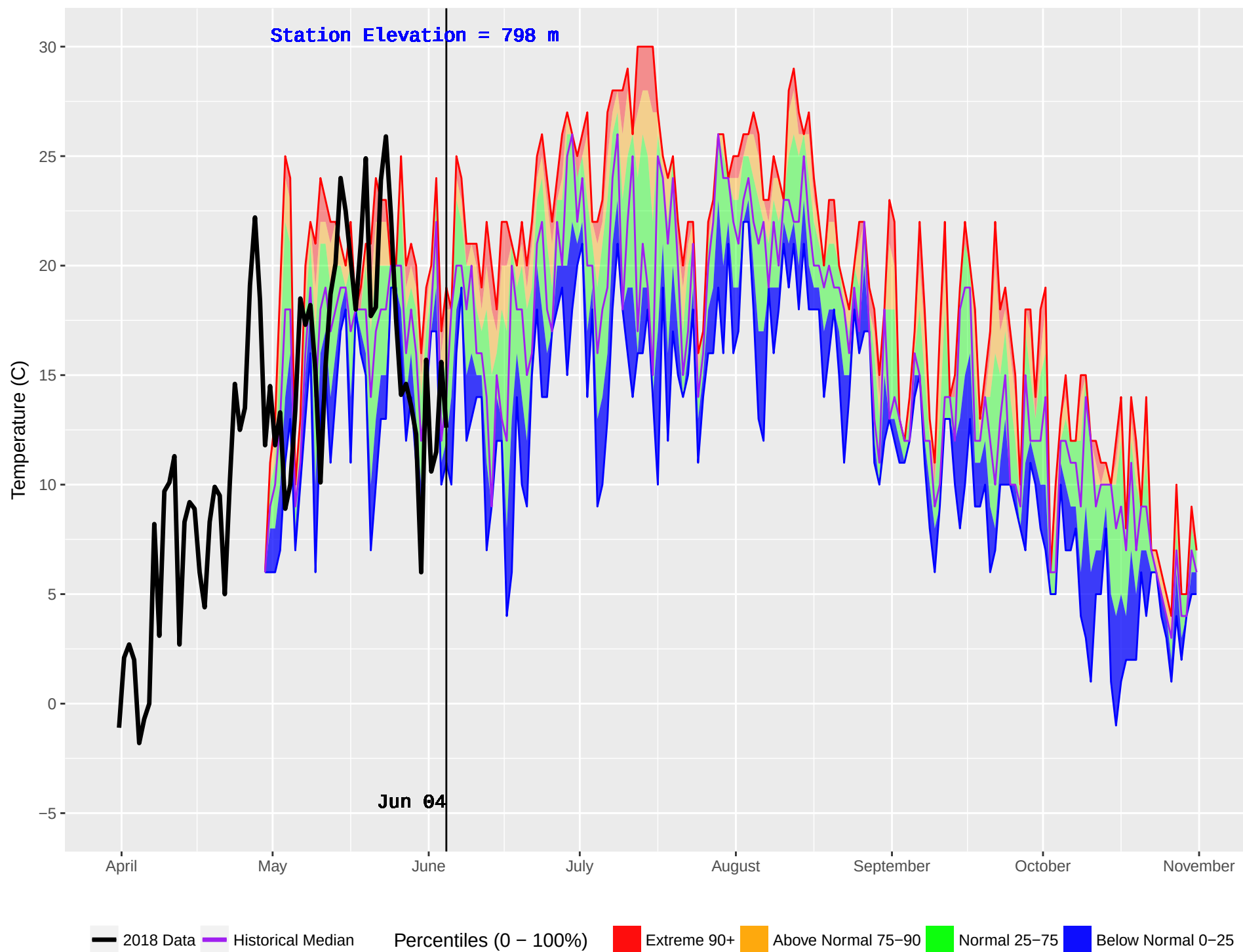
SEVEREID (1165) : Historical (2014–2016) and Current (2018) Noon Temperature
